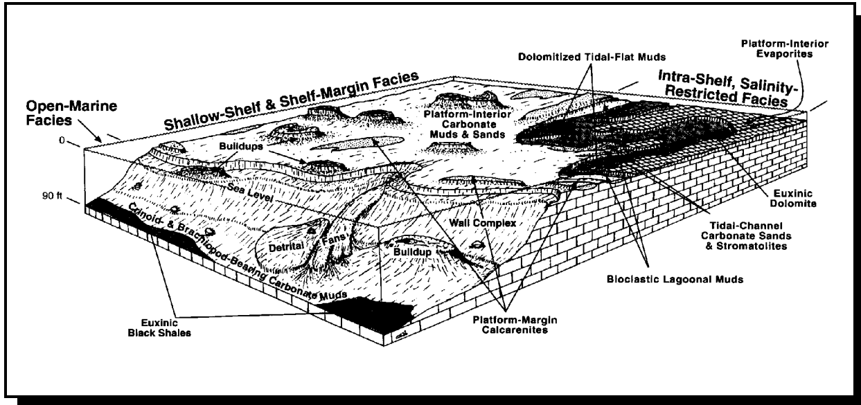
Figure 3.1. Block diagram displaying major facies within regional facies belts for the Desert Creek zone, Pennsylvanian Paradox Formation, southeastern San Juan County, Utah (from Chidsey and others, 1996f).
