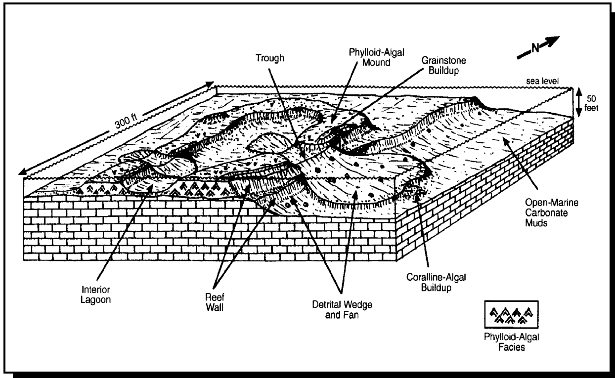
Figure 2.3. Block diagram displaying depositional interpretation of Wild Horse Canyon mound complex and associated features (from Chidsey and others, 1996a). This interpretation is a composite of inferences made from outcrop and subsurface data.
