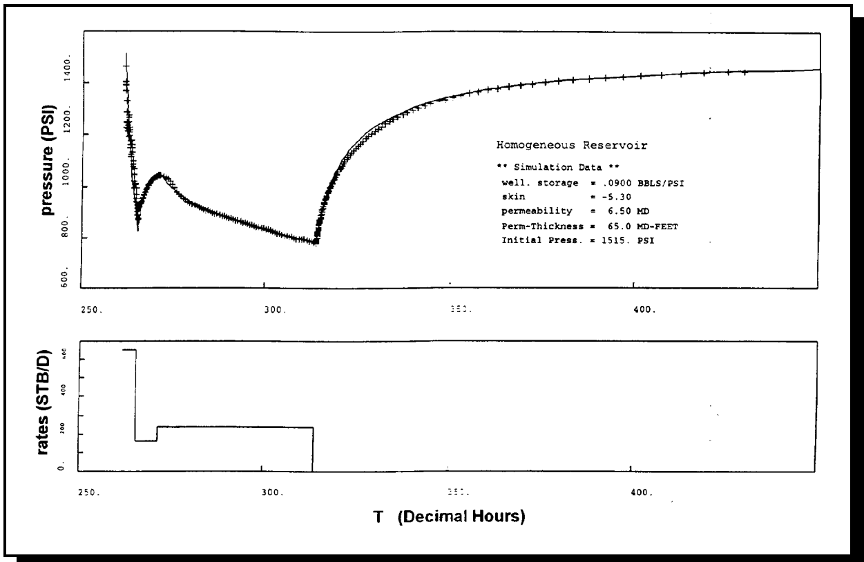
Figure 5.3. Well flow buildup test analysis of the Big Sky No. 6E well near Clay Hill field (see figure 1.1) displaying pressure vs. time match.
