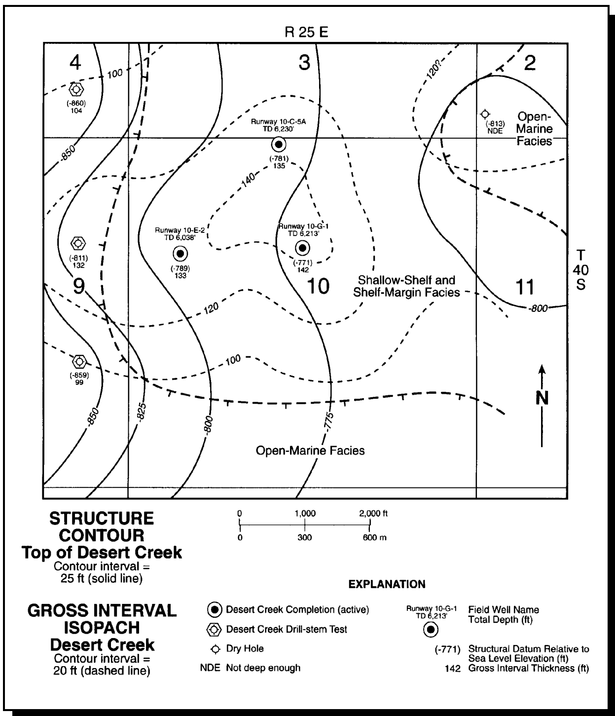
Figure 3.8. Combined Desert Creek zone structure contour and gross interval isopach map, Runway field, San Juan County, Utah, Navajo Nation (from Chidsey and others, 1996e). Hachured lines separate carbonate depositional facies.
