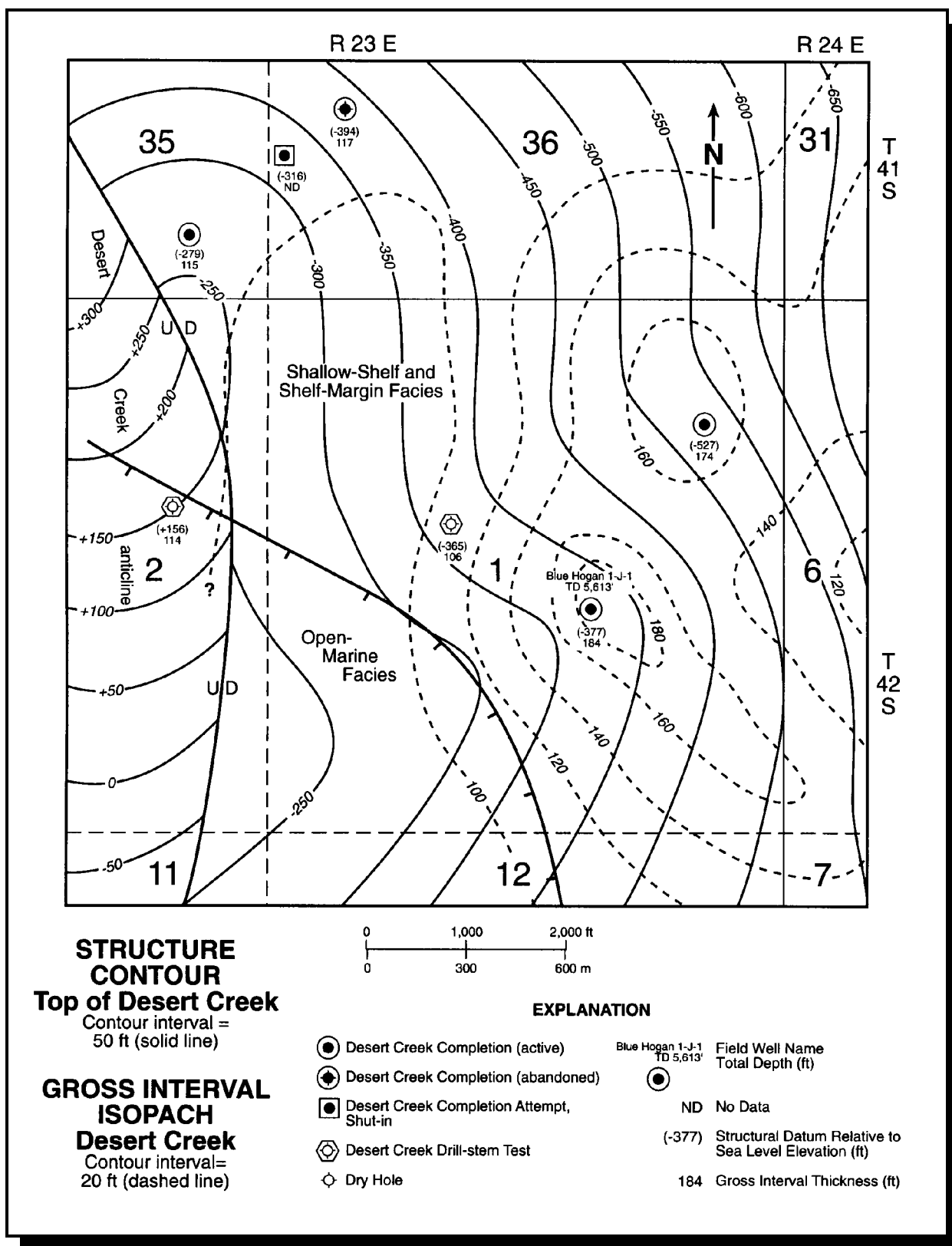
Figure 3.5. Combined Desert Creek zone structure contour and gross interval isopach map, Blue Hogan field, San Juan County, Utah, Navajo Nation (from Chidsey and others, 1996b). Hachured lines separate carbonate depositional facies.
