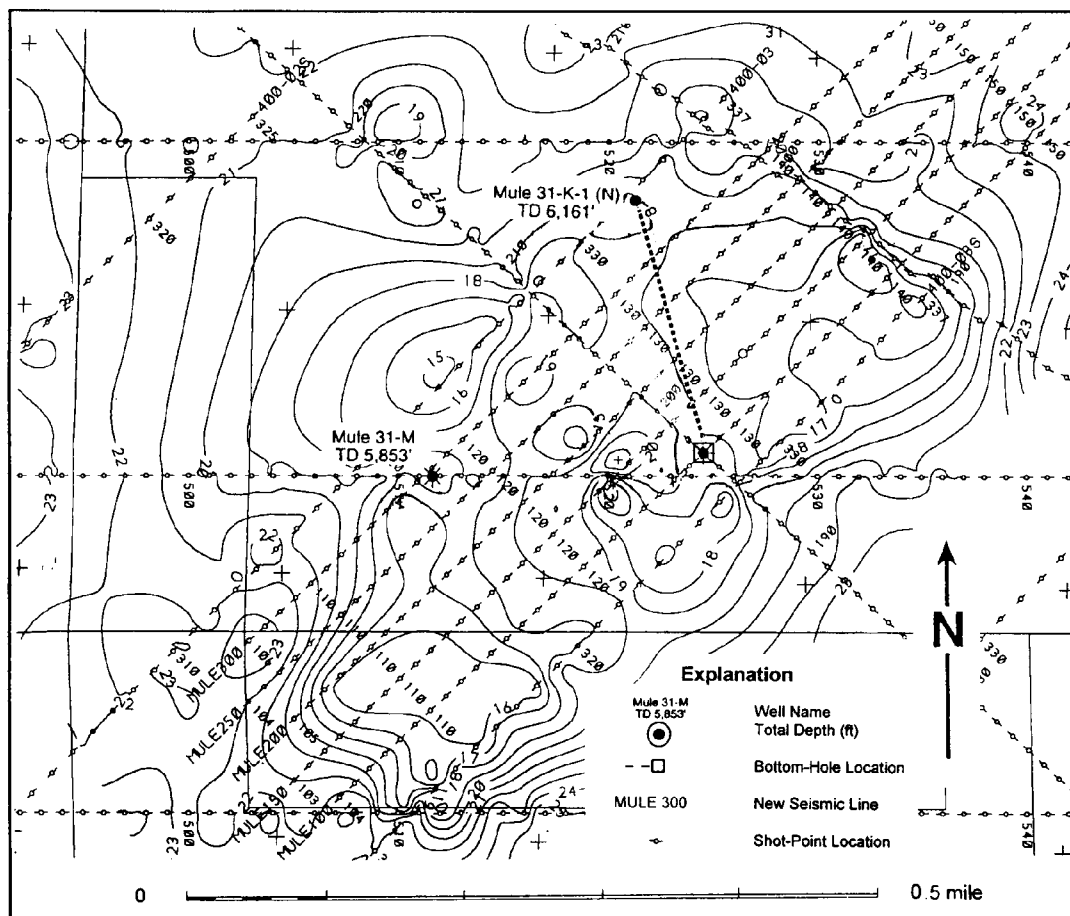
Figure 3.10. Ismay zone to Desert Creek zone (Pennsylvanian Paradox Formation) isochron map, Mule field area. Contour interval = 1 millisecond.
