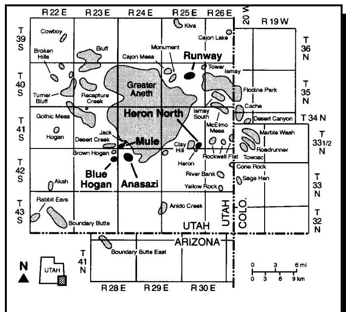
Figure 1.1. Shallow-shelf carbonate fields (the five project fields are indicated by dark shading with names in bold type) in the Paradox basin, Navajo Nation, San Juan County, Utah are targeted for geological and reservoir characterization.
