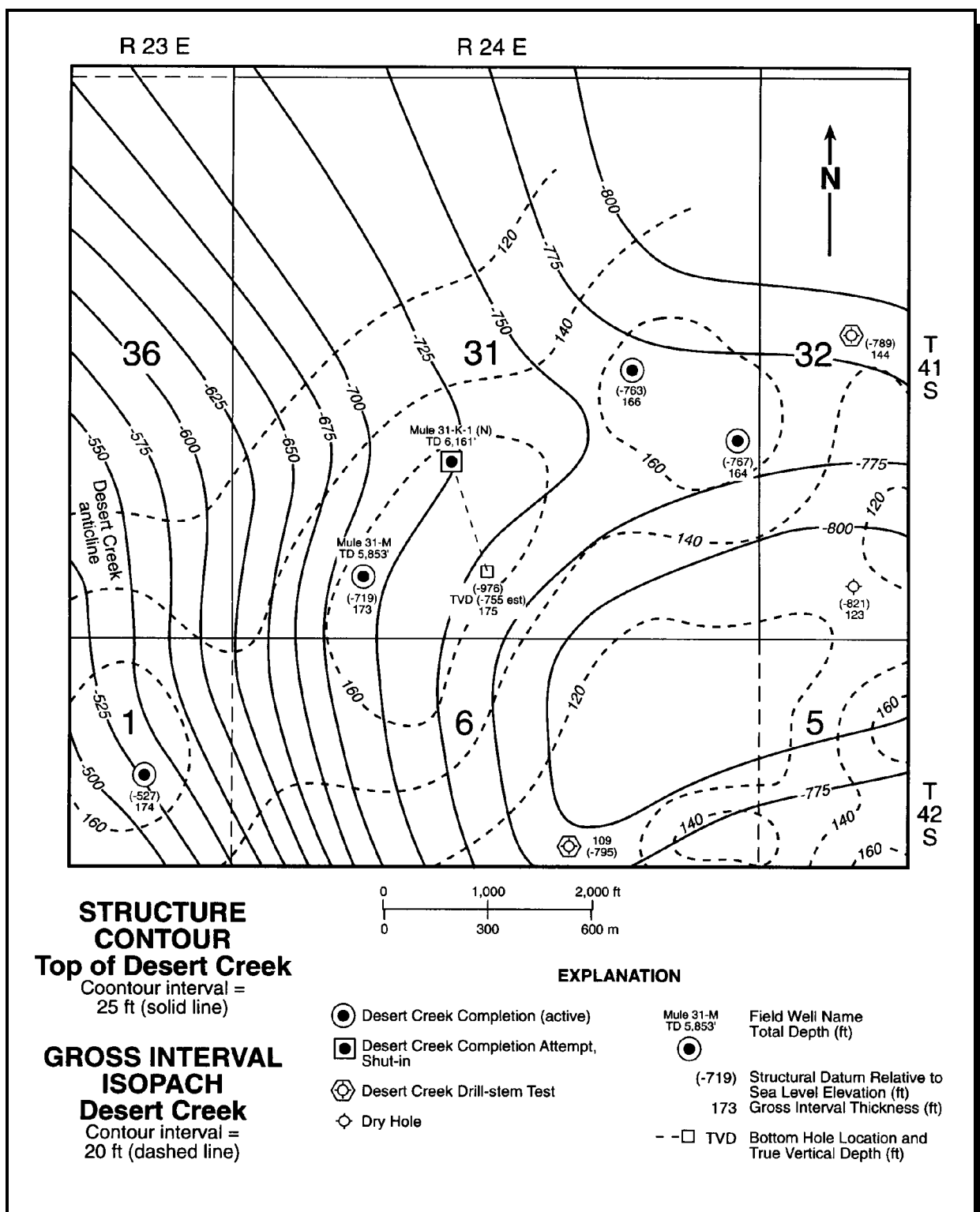
Figure 3.7. Combined Desert Creek zone structure contour and gross interval isopach map, Mule field, San Juan County, Utah, Navajo Nation (from Chidsey and others, 1996d).
