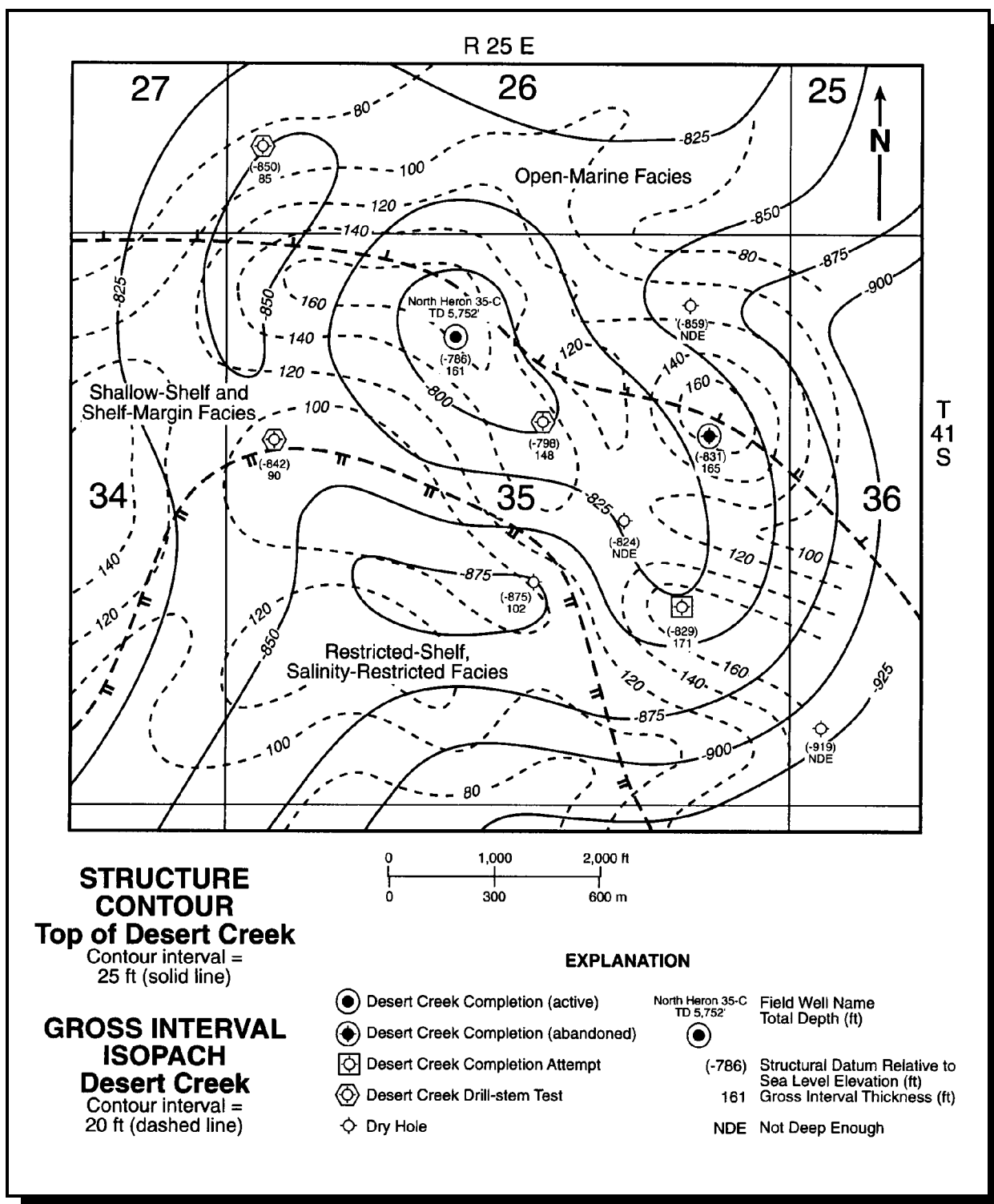
Figure 3.6. Combined Desert Creek zone structure contour and gross interval isopach map, Heron North field, San Juan County, Utah, Navajo Nation (from Chidsey and others, 1996c). Hachured lines separate carbonate depositional facies.
