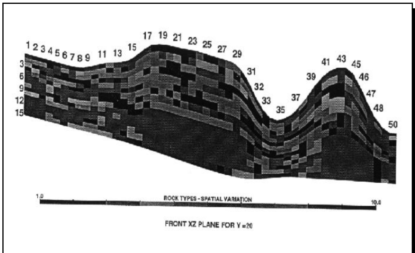
Figure 4.3. Cross section, through the Anasazi No. 1 well, of the 15-layer geostatistical Anasazi reservoir simulation model displaying the spatial distribution of lithotypes.
