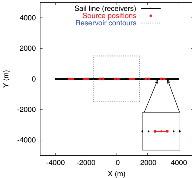
Figure 3. Inversion 1: Transmitter–receiver configuration for synthetic data generation of a single-profile seafloor survey.
