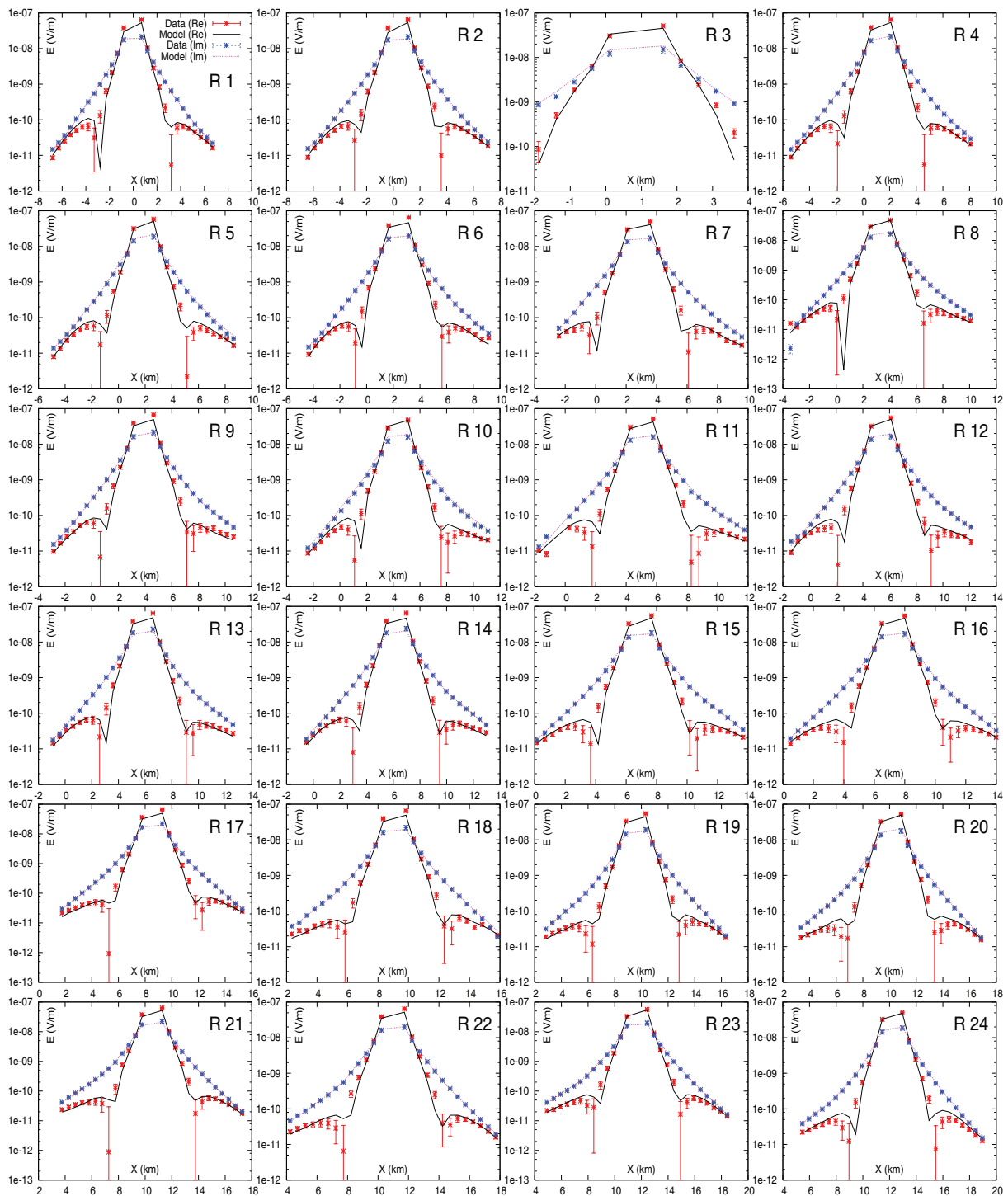
Figure 19. Data fits for TWGP inversion. Shown are observed and reproduced electric fields along the receiver profile for each source R1–R24 using the transmitter frequency f_1 = 0.25 Hz. The red and black curves are the real parts of the observed and reproduced electric field, respectively. The blue and purple curves are the corresponding imaginary parts.
