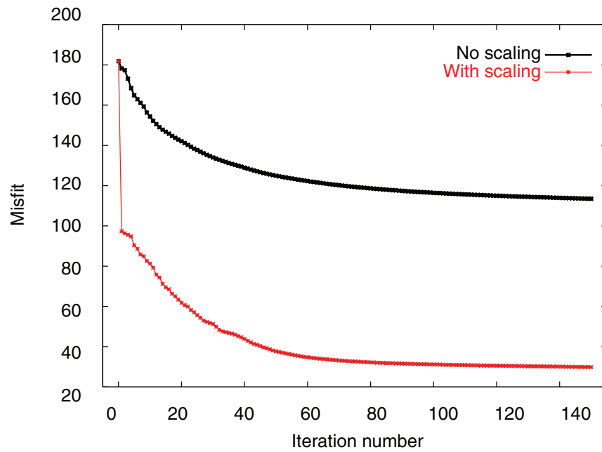
Figure 12. Inversion 4: Error functional \Phi for data inversion without (black) and with (red) source signature correction factor.
