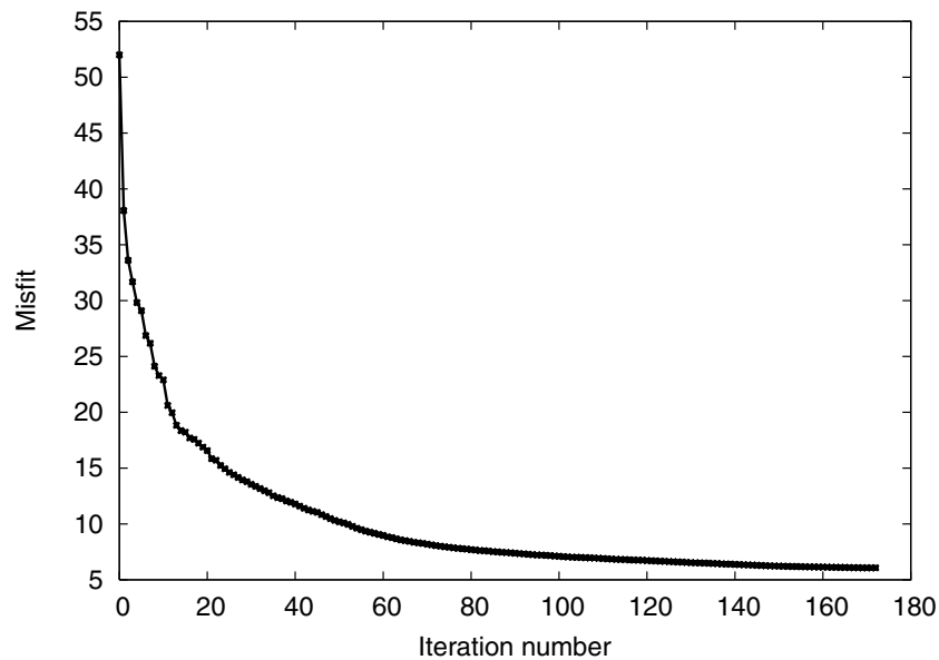
Figure 18. Error functional \Phi of the TWGP inversion.
