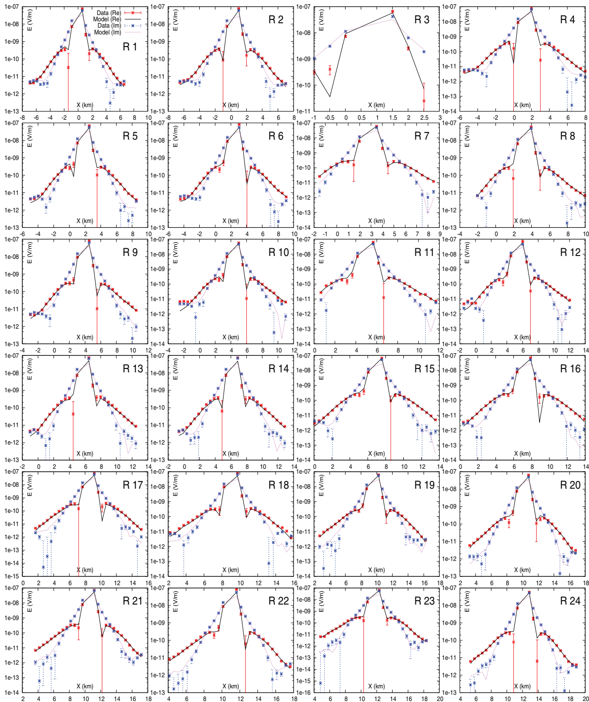
Figure 20. Data fits for TWGP inversion. Shown are observed and reproduced electric fields (real and imaginary parts) for each source R1–R24 using the transmitter frequency f_2 = 0.75 Hz.
