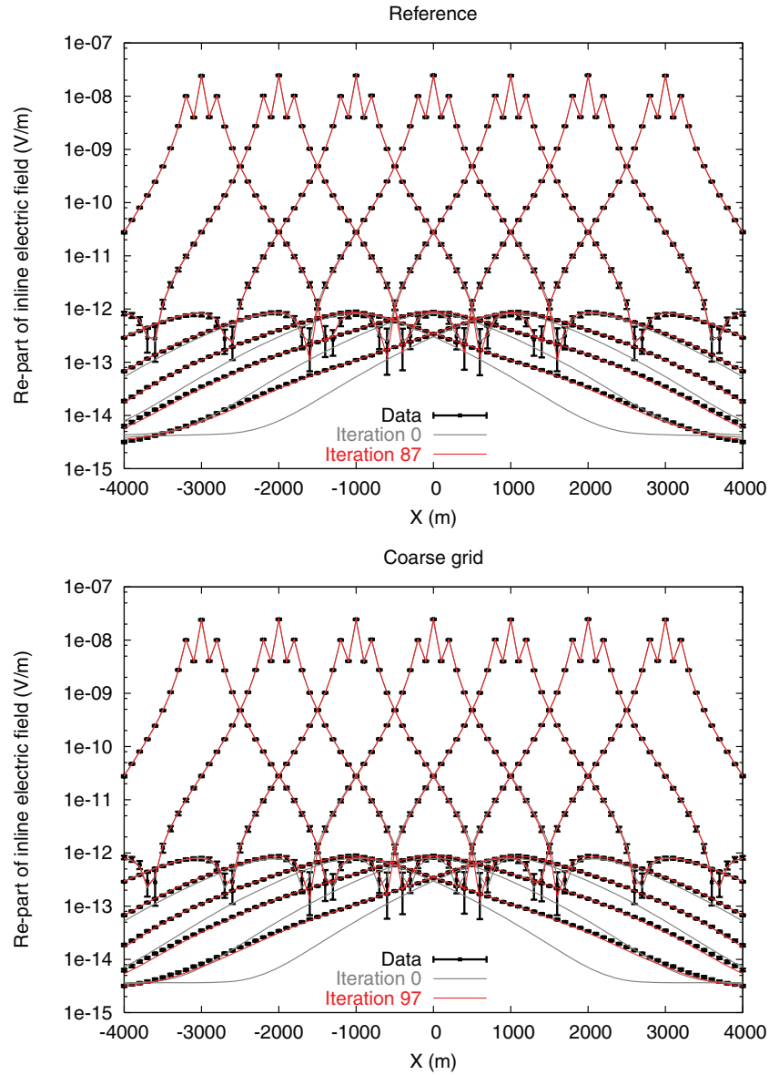
Figure 5. Inversion 1: Data fits for all seven sources (survey configuration shown in Fig. 3), exemplified for the excitation frequency f = 0.25 Hz. Initial (grey) and final fits (red) for both reference and coarse-grid inversions are shown.
