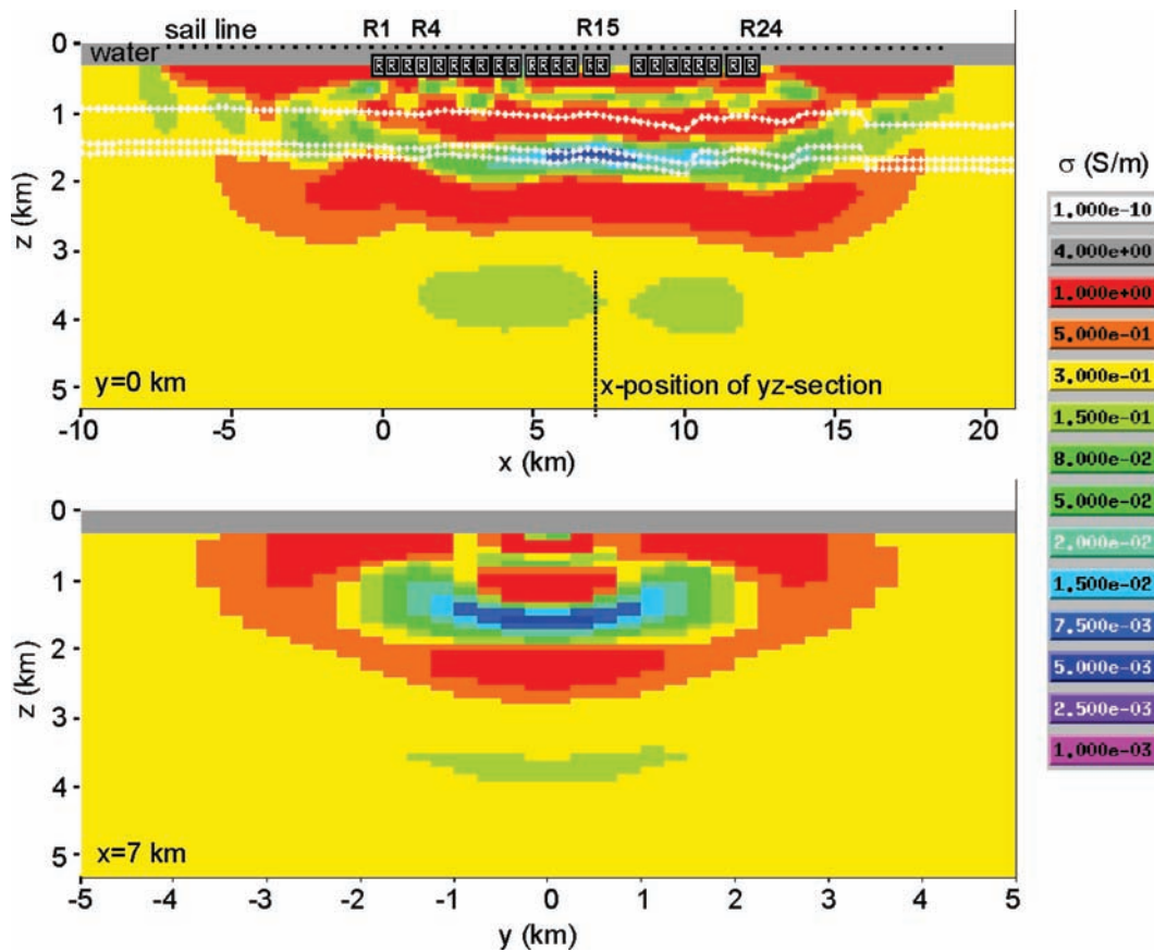
Figure 21. Final imaging result of TWGP inversion. R1–R24 mark the source positions projected to the xz -plane. The white lines in the upper figure represent interpreted seismic reflection horizons (Hoversten et al. 2006).
