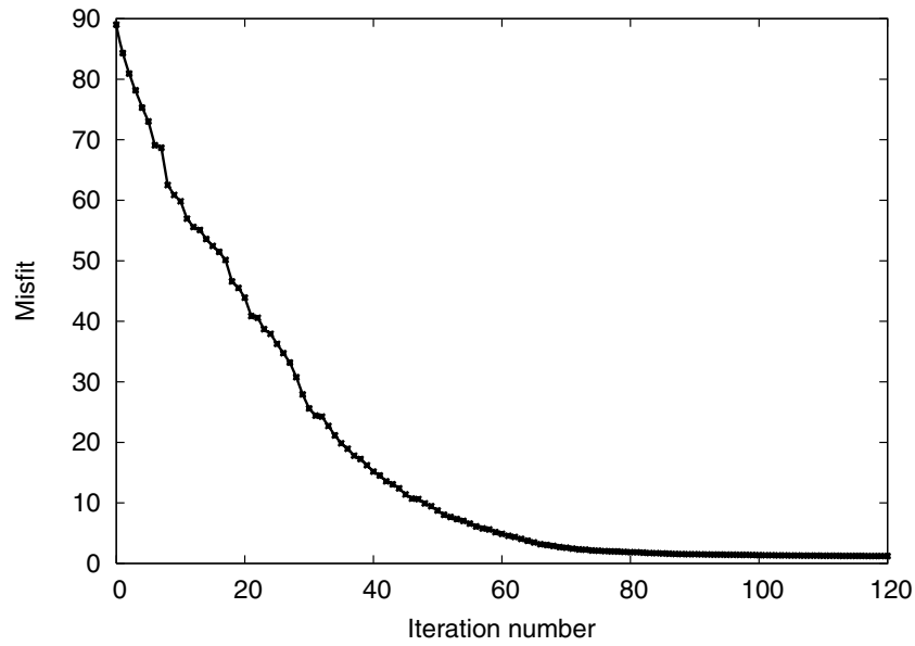
Figure 10. Inversion 3: Error functional \Phi , according to eq. (1), of synthetic multiprofile data inversion.
