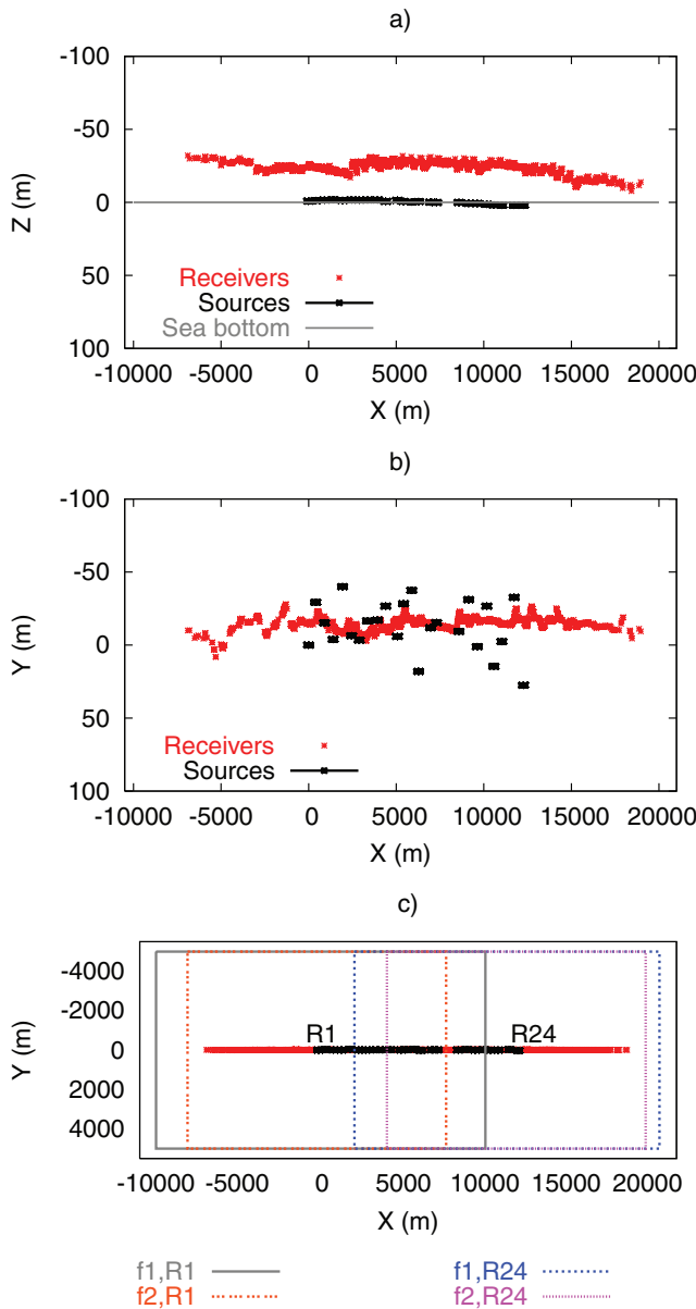
Figure 17. Layout of the survey over the Troll West Gas Province. (a) Vertical section ( xz ). (b) Horizontal section ( xy ). (c) Illustration of the model subdomains covered by the simulation grids assigned to sources R1 and R24 for both frequencies f_1 and f_2 .
