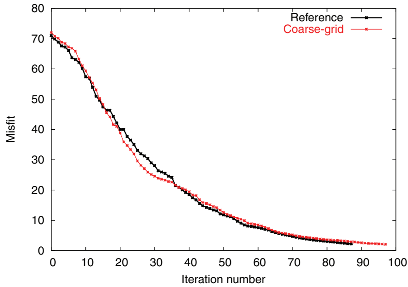
Figure 4. Inversion 1: Error functional \Phi , according to eq. (1), of synthetic single-profile data inversion.
