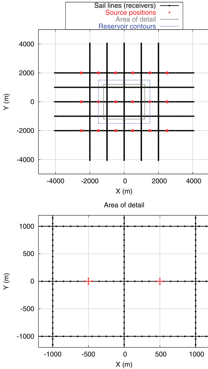
Figure 9. Inversion 3: Transmitter-receiver configuration of 3-D seafloor survey with grid layout.
