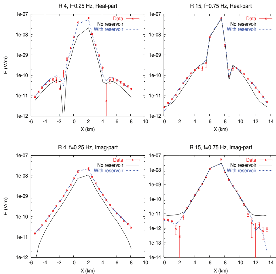
Figure 23. Data fits produced from TWGP inversion (blue curves) in comparison with a non-reservoir model (black curves), exemplified for the source positions R4 and R15 and both frequencies f_1 = 0.25 Hz and f_2 = 0.75 Hz.
