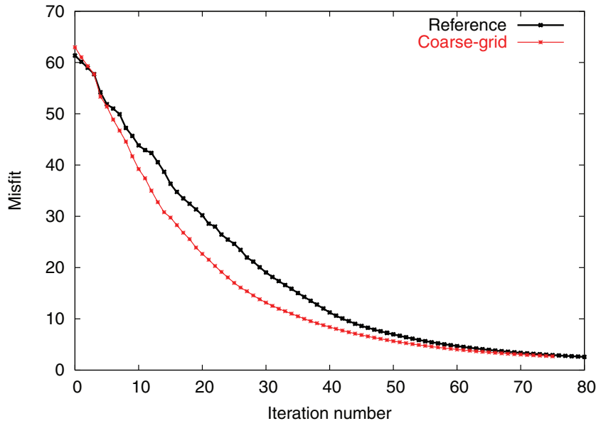
Figure 7. Inversion 2: Error functional \Phi , according to eq. (1), of synthetic single-profile data inversion.
