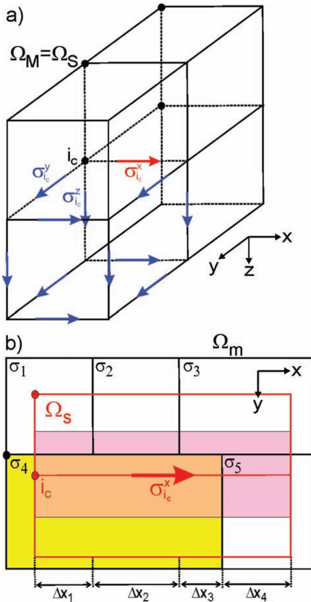
Figure 1. Illustration of scheme for mapping between model and simulation grid. (a) shows the equal-grid case. (b) illustrates the case of different grids in two dimensions.
