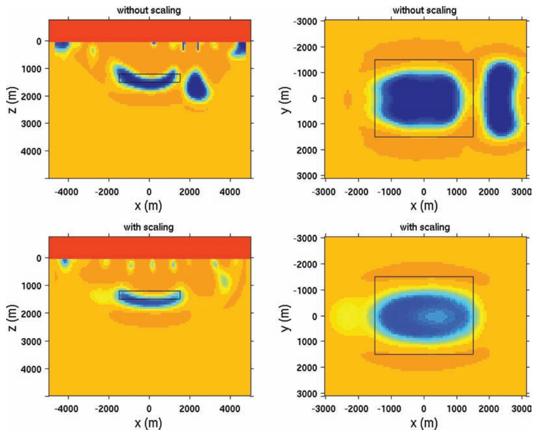
Figure 13. Inversion 4: Final model solution for inversion of data set with distorted transmitter endpoint positions. Upper/lower figures are created from inversions without/with source signature correction factor as an additional inversion parameter.
