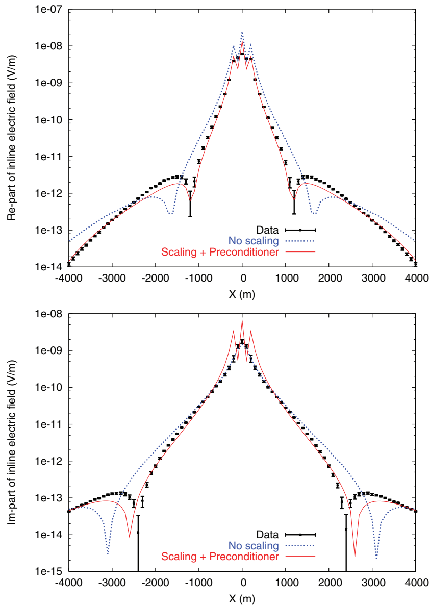
Figure 15. Inversion 5: Data fits exemplified for the source centred at x = 0 m of the survey configuration shown in Fig. 3. The excitation frequency is f = 0.25 Hz. The inverted data is given by the black symbols. Data computed from the inversion result are shown for the case without using SSC (blue) and for the case using both SSC and PC (red).
