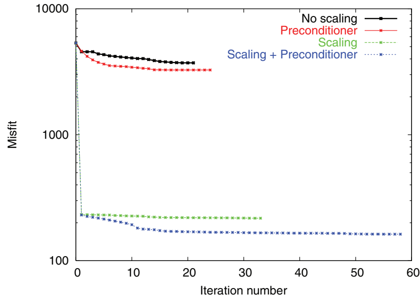
Figure 14. Inversion 5: Error functional \Phi for inversion of distorted data without SSC factor and PC activated (black). Red, green, and blue curves show results when PC, SSC and both PC and SSC are active, respectively.
