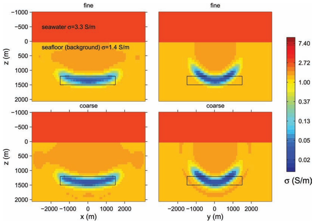
Figure 8. Inversion 2: Final model solution for reference (upper) and coarse-grid (lower) inversions.
